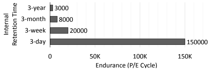
Fig. 1. P/E cycle endurance from different amounts of internal retention time without refresh. (Data extrapolated from prior work [9, 10].)
