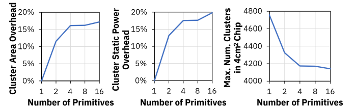
Fig. 20: Area (left) and static power (center) overheads for supporting multiple primitives in 1S1R, normalized to single-primitive 1S1R; maximum number of 1S1R clusters that can fit in a 4 cm 2 chip (right).
