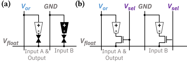
Fig. 13: (a) Voltage assertions for 1S1R OSCAR OR; (b) voltage assertions for 1T1R OSCAR OR.
